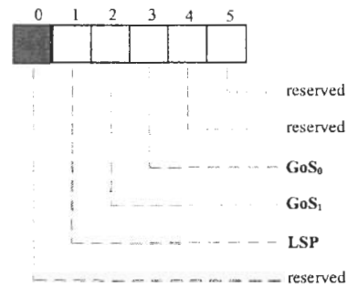
Fig. 4. Some bits unused in the TCP header.
