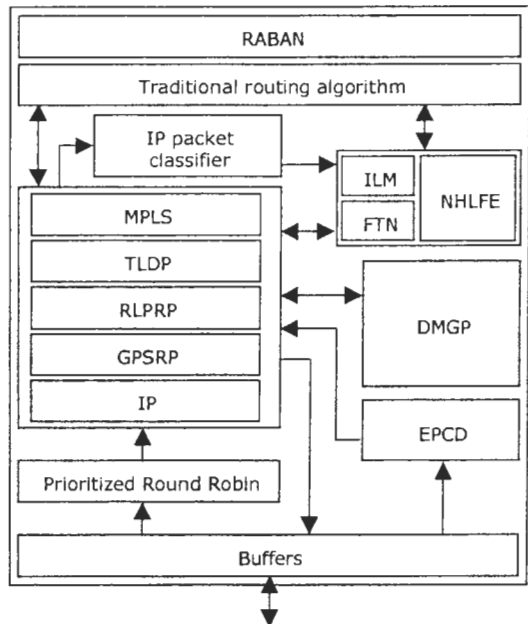
Fig. 3. Internal architecture of an active node with routing features.
