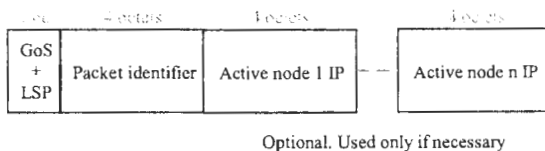
Fig. 5. Proposed format for the IP options field.
